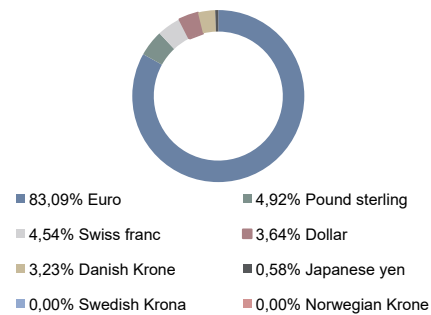
Currency exposure
