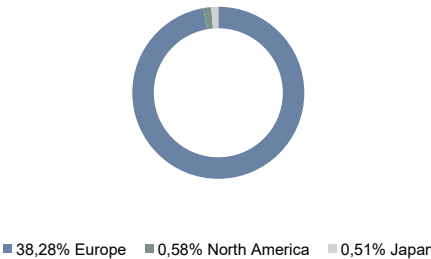
Equity distribution
